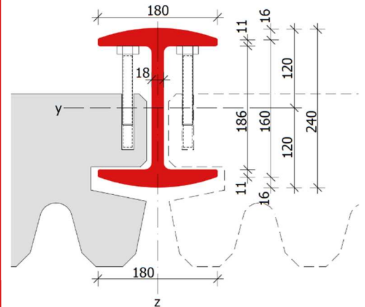
Post cross-section in mm
